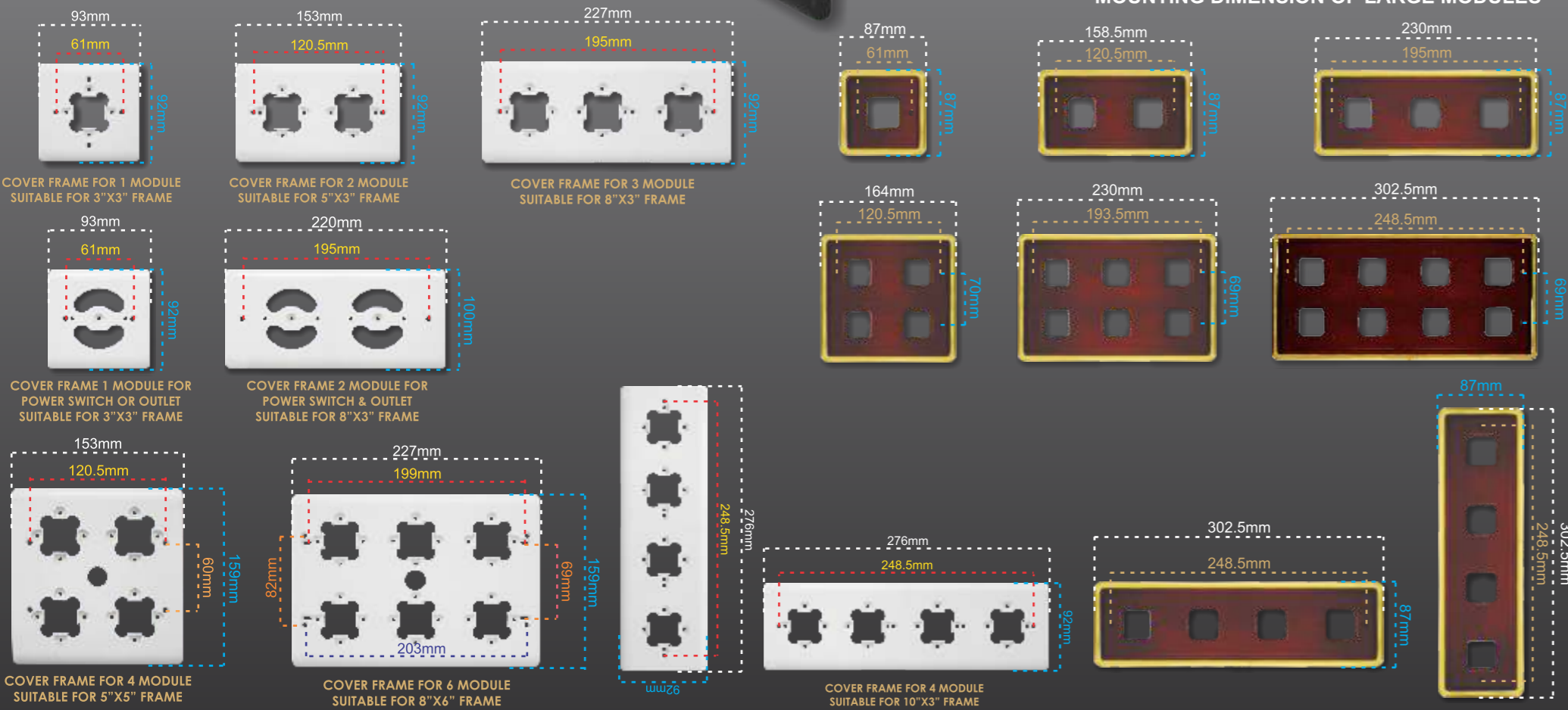
MOUNTING DIMENSION OF LARGE MODULES
