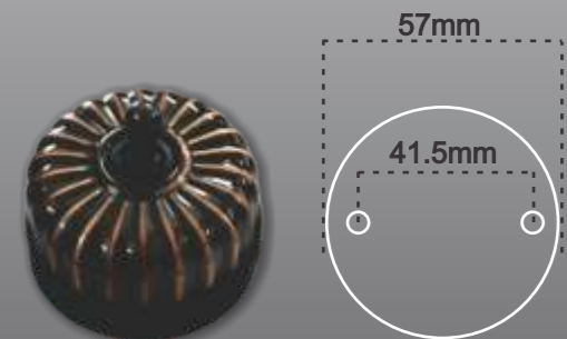
MOUNTING DIMENSION OF ALL MODULES
